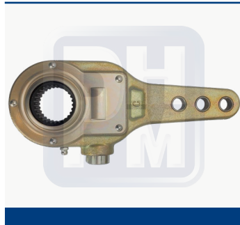
Matraca fina 1.50"-28 ranuras 5, 6, 7 drilling 5 rivet heavy duty
