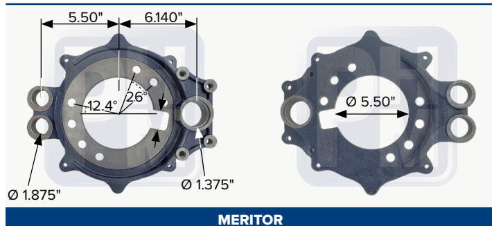
Araña porta zapatas
