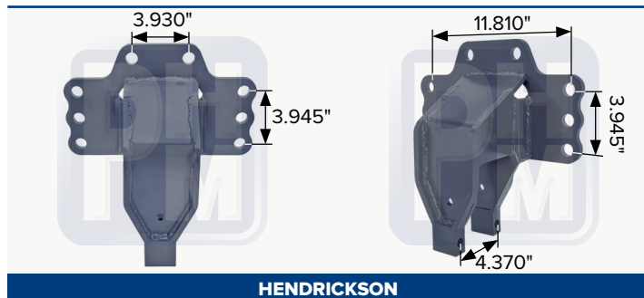
OEM 97334A00 Percha trasera
