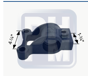
OEM 0305117, M1641 Terminal de muelle larga
